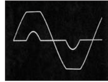
Oscillograph of voltage and current waveform at load due to distribution losses. THD=6.6%
